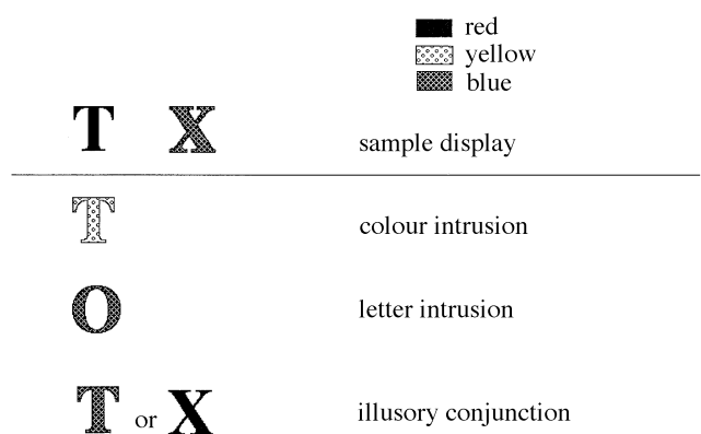
Figure 2. Stimuli used to test feature binding in patient R.M.
