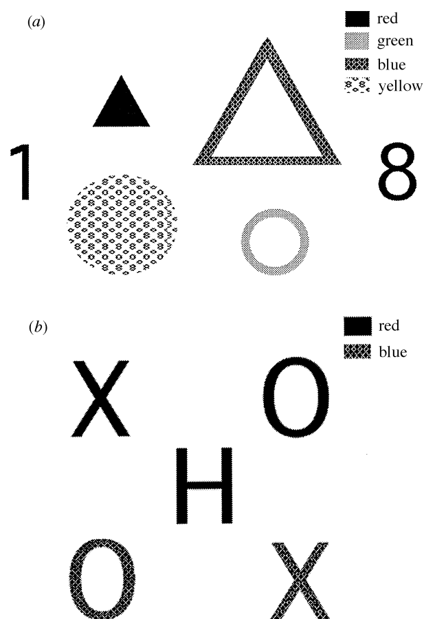
Figure 3. (a) Display illustrating task to test the role of attention in binding in normal subjects. The task is to report the identity of the two digits first and then as many features as are confidently seen for the object in the cued location, indicated by the bar marker. (b) Display illustrating same–different matching task that reveals binding errors without a load on memory.
